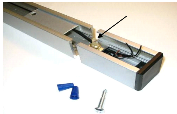
Optional Bypass Switch - PT Mount
