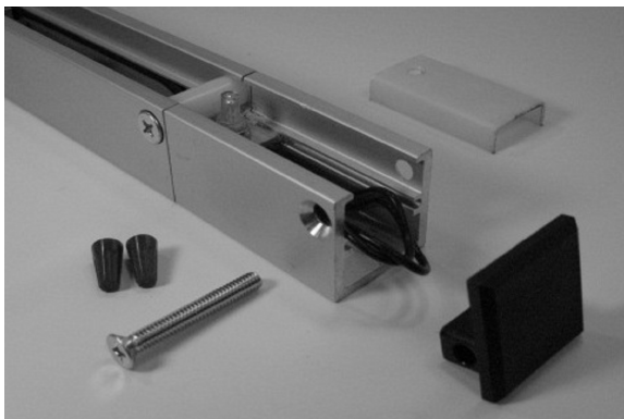
Optional Track Bypass Switch - T Mount
